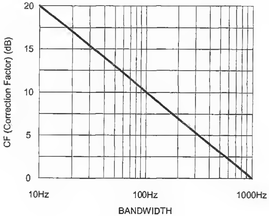
Figure 13-3 (U) Bandwidth Correction Factor (U)
